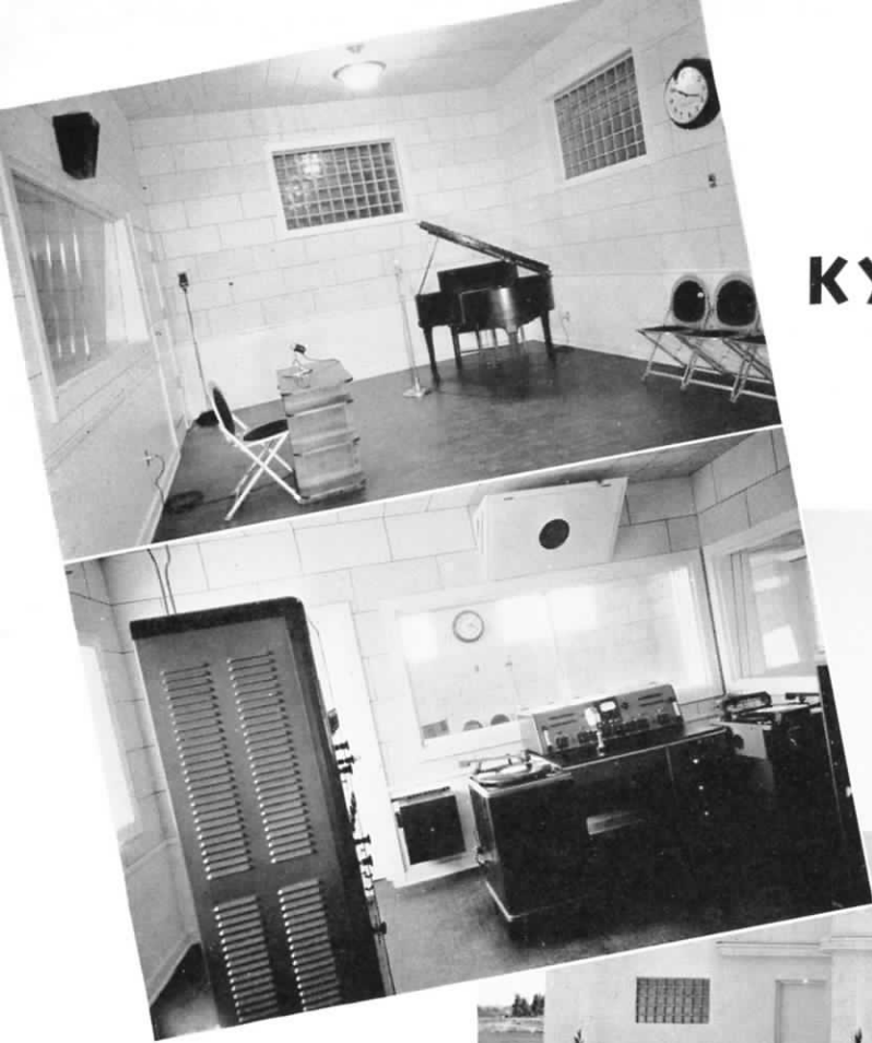
▲ TOP: One of the well arranged studios at KYUM. LOWER: RCA transmitter, turntables and console form an efficient set-up.
