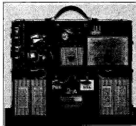
Fig. 1. Rear view of battery supply cabinet used with 30-A equipment. Note how small amplifier fits into compartment. Also note space for accessories.
