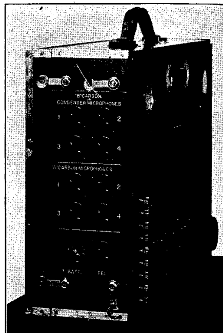
Fig. 3. End view of 30-A portable amplifier showing the two groups of microphone receptacles.
