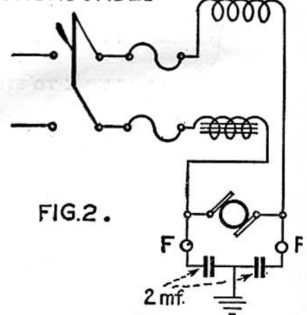
The choke coil consists of 100 turns of No. 18 D.C.C. wire wound in a single layer on a 3-inch tube form, 1/8-inch thick and 8 inches long. It is wrapped with insulating tape after winding.
