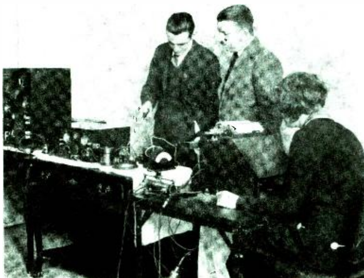
Mr. W. G. H. Finch demonstrating his radio-controlled typewriter designed for rapid news service to Mr. Laurence M. Cockaday, famous radio engineer. Mr. Finch is pointing to the highly sensitive relay, the heart of the mechanism.
