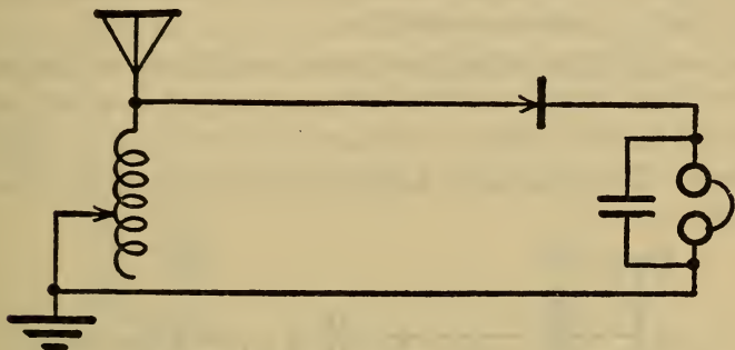
EXAMPLE OF DIRECT COUPLING.
