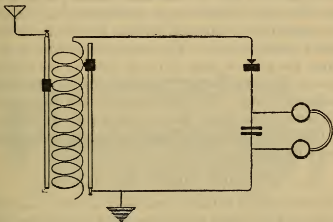
CIRCUIT OF RADIO RECEIVING SET WITH DOUBLE SLIDE TUNING COIL, CRYSTAL DETECTOR AND SIMPLE CONDENSER.
