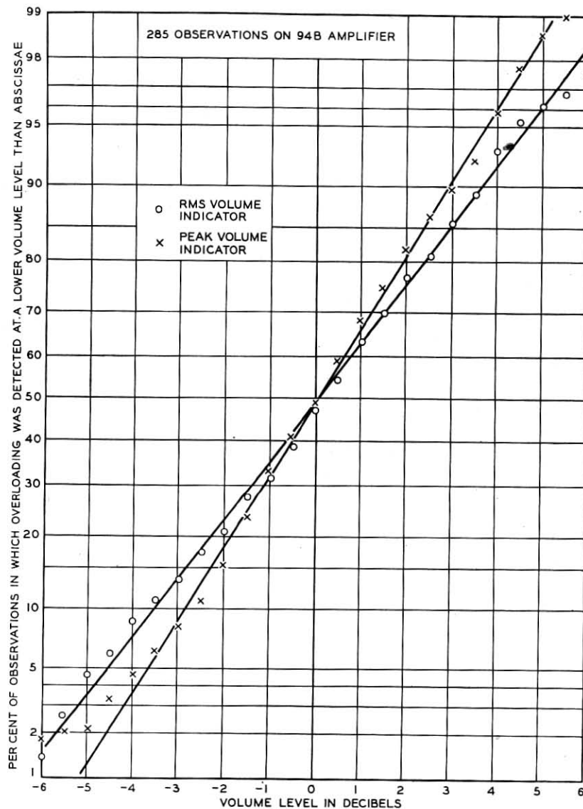
Fig. 5—Comparison of peak vs. r-m-s volume indicators as overload indicators (using W.E. 94B amplifier).
