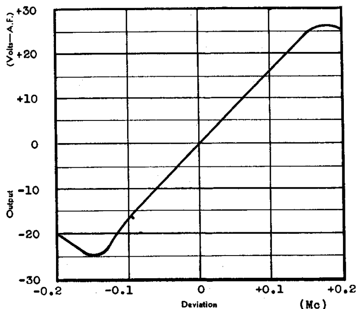
Characteristic of Demodulator Fig. 3
