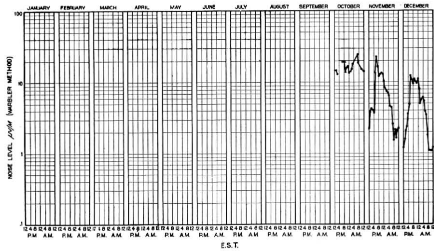
Monthly Average of Diurnal Variation of Noise Green Harbor, Mass., 1923 34,000 Cycles
