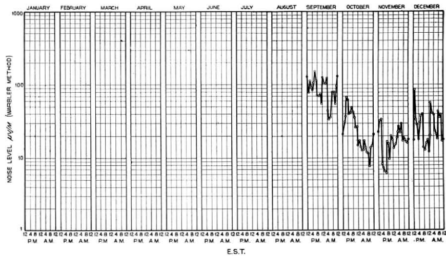
Riverhead, L. I. Monthly Average of Diurnal Variation of Noise 15,000 Cycles 1924
