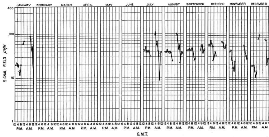
Monthly Average of Diurnal Variation of Signal Field Strength Leafield, England (GBL) Measured at Green Harbor, Mass. Corrected to 300 Amperes Antenna Current 5,150 Km. 24,050 Cycles July, 1923—Jan., 1924
