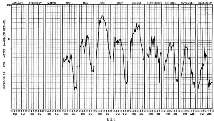
Belfast, Maine Monthly Average of Diurnal Variation of Noise 52,000 Cycles 1924
