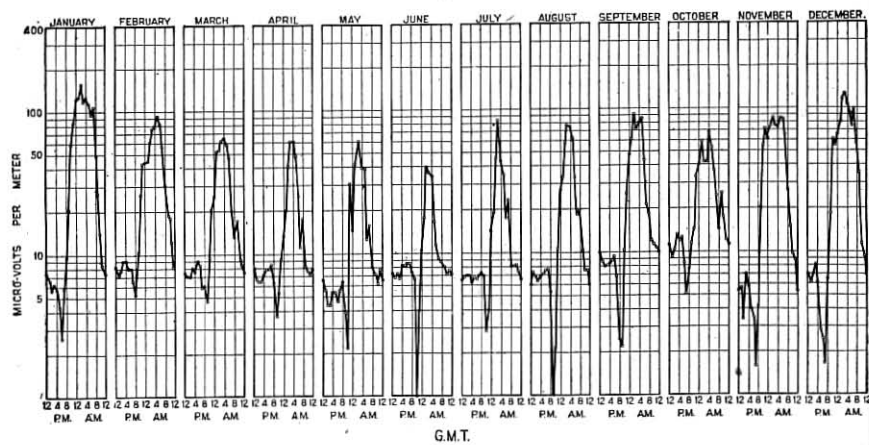
Monthly Averages of Diurnal Variation of Signal Field Strength Rocky Point, L. I., U. S. A. (2XS) Measured at New Southgate, England Corrected to 300 Amperes Antenna Current 5,480 Km. Jan., 1923—Dec., 1924 57,000 Cycles
