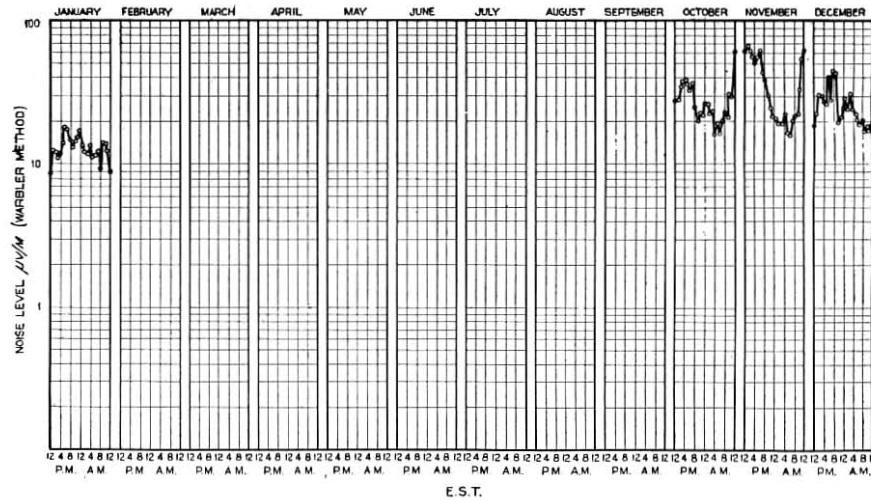
Monthly Average of Diurnal Variation of Noise Green Harbor, Mass. 15,000 Cycles Oct., 1923—Jan., 1924
