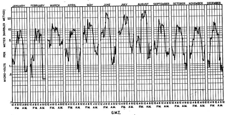
Monthly Averages of Diurnal Variation of Noise New Southgate, England Oct., 1923—Feb., 1925 37,000 Cycles
