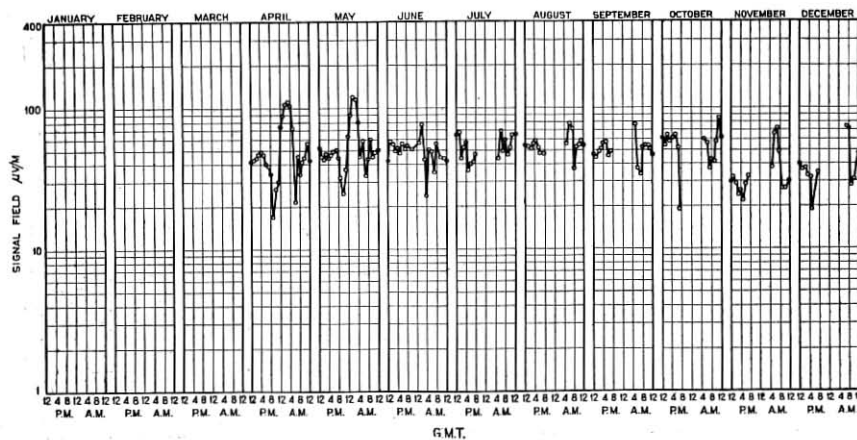
Monthly Averages Diurnal Variation of Signal Field Strength Leafield, England (GBL) Measured at Belfast, Maine Corrected to 300 Amperes Antenna Current 4,980 Km. 1924 24,050 Cycles
