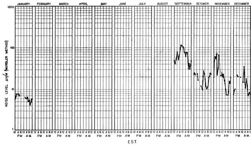
Monthly Average of Diurnal Variation of Noise Green Harbor, Mass. Sept., 1923—Jan., 1924 24,000 Cycles
