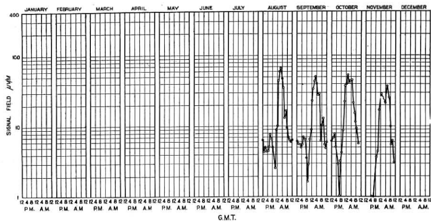
Monthly Averages Diurnal Variation of Signal Field Strength Northolt, England (GKB) Measured at Riverhead, L. I. 5,460 Km. 52,000 Cycles 1924
